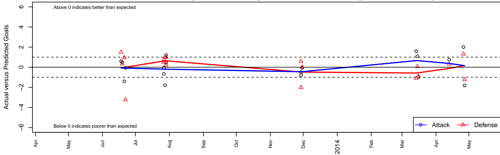
FRAM Premier B95 Dots are actual minus expected GF (blue circles) and GA (red triangles). Blue line is smoothed change in attack strength. Red is smoothed change in defense strength.
